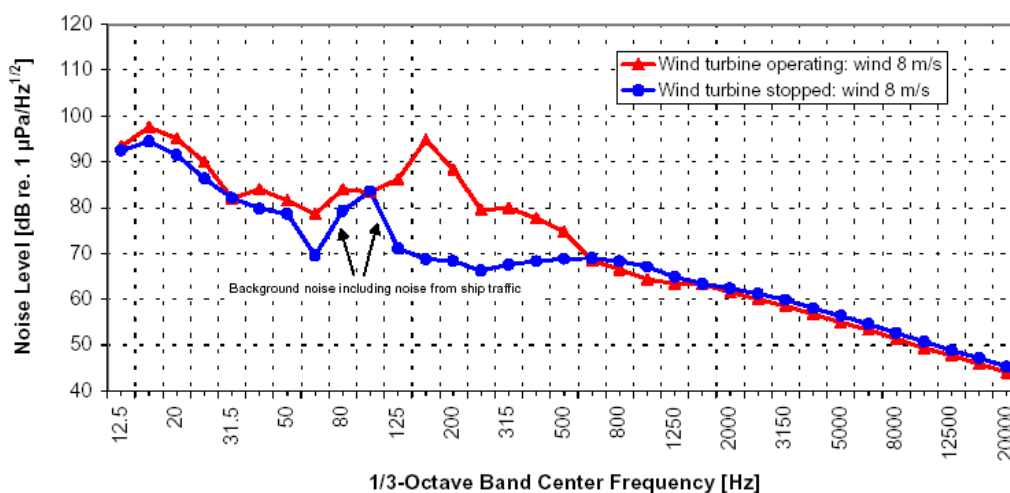
Fig. 11: Underwater noise emitted from a single offshore turbine (550 kW) at Gotland and respective background noise. Levels are recorded at a distance of 20 m from the turbine and are plotted in \frac{1}{3} octave bands with linear averaging over 4 to 5 minutes (from: DEGN 2000).
