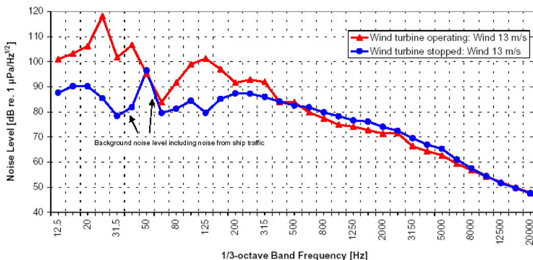
Fig.10: Underwater noise emitted from a single offshore turbine (450 kW) at Vindeby and respective background noise. Levels are recorded at a distance of 14 m from the turbine and are plotted in \frac{1}{3} octave bands with linear averaging over 4 to 5 minutes (from: DEGN 2000).
