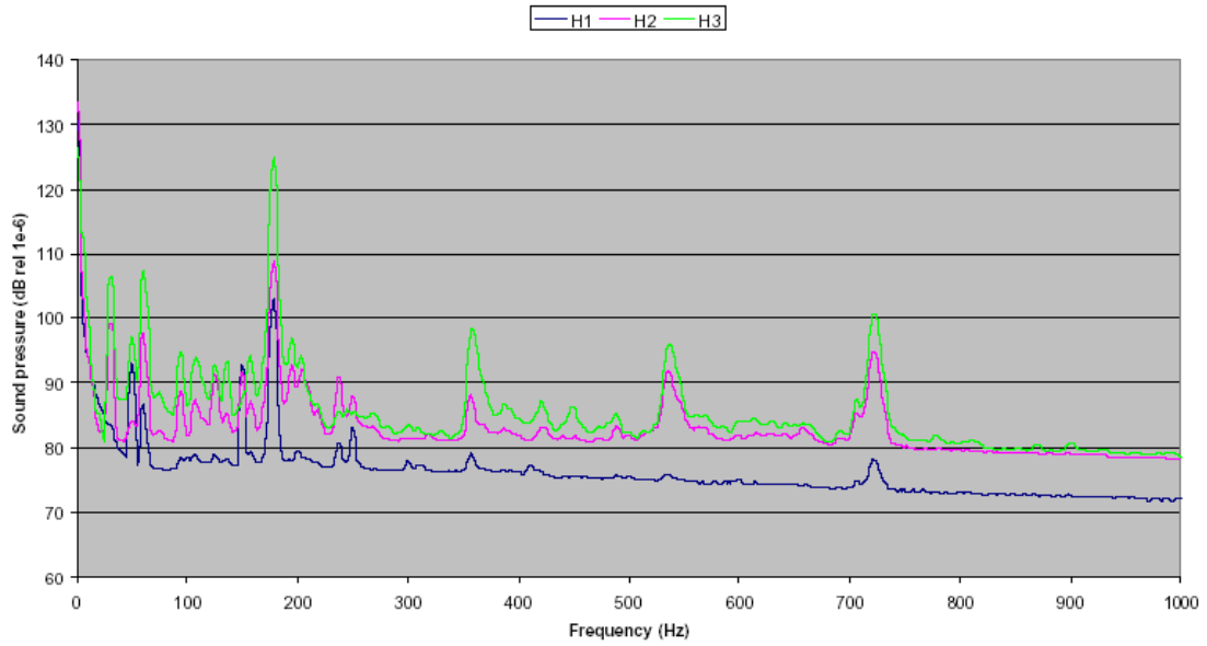
Fig. 15: Sound measured at turbine 4 at high wind conditions (11 to 14 m/s, east) plotted for the different hydrophone positions 463 m, 160 m and 83 m distance (from: INGEMANSSON TECHNOLOGY 2003).
