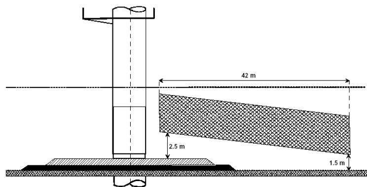
Figure 10: Sampling design of anchored gillnet catches on selected wind turbine foundations at Horns Rev (from LEONHARD & PEDERSEN 2004).
