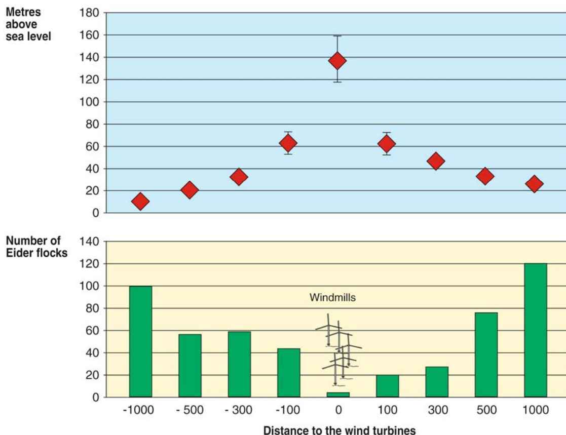
Fig. 8: Flight altitudes (top; mean and standard deviation) and number of flocks (bottom) recorded at various distances from Ytre Stengrund wind farm during autumn migration of Eiders (September 2002). Total turbine height is 96 m; from PETERSSON & STALIN 2002.
